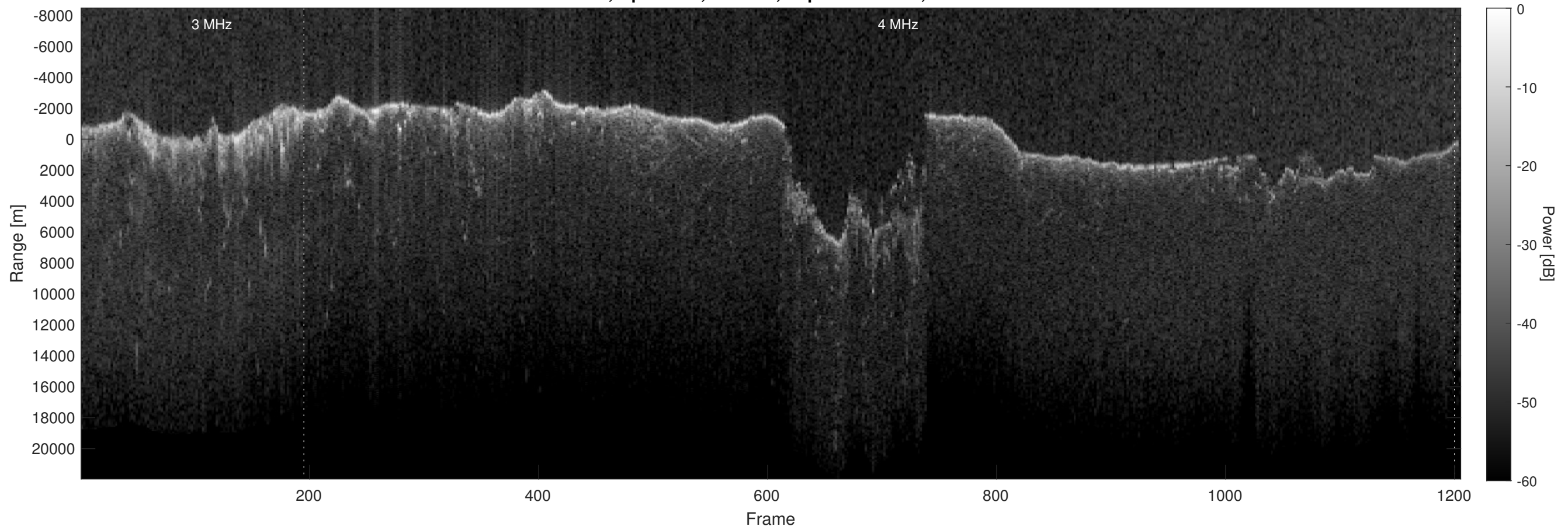
Orbit 6223, Optimized, Window, Depth-Corrected, Channel 2
