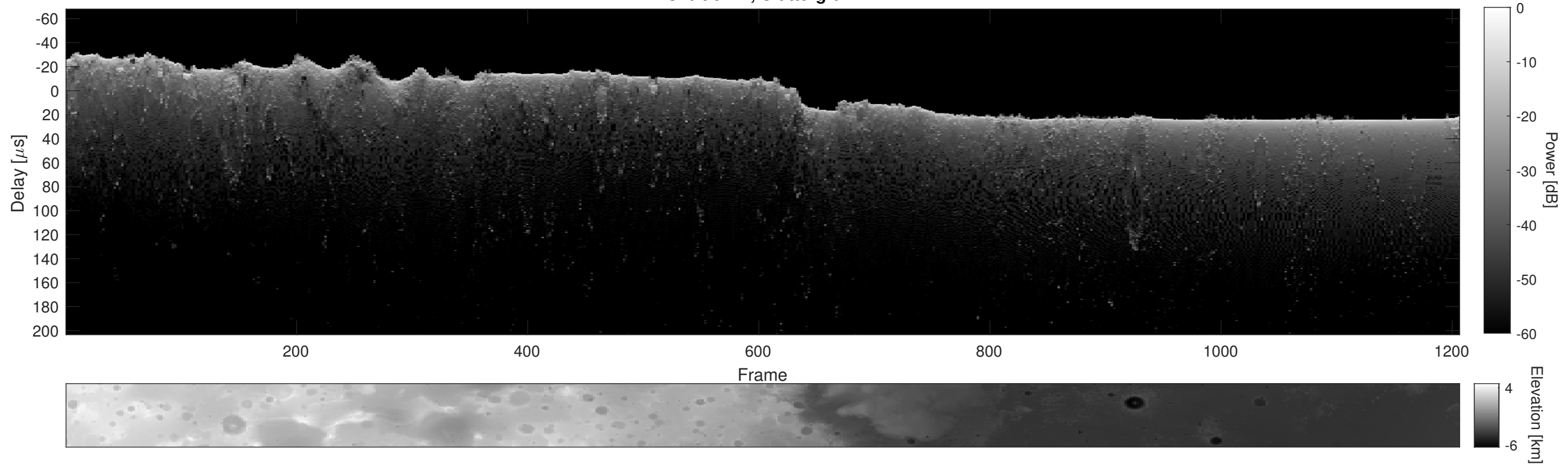
Orbit 6224, Cluttergram
