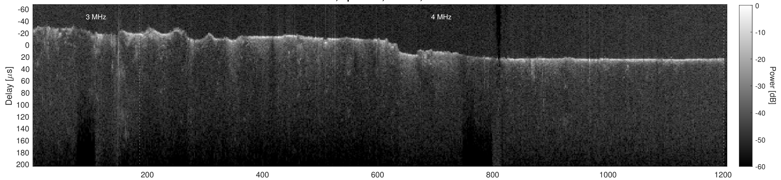
Orbit 6224, Cluttergram
