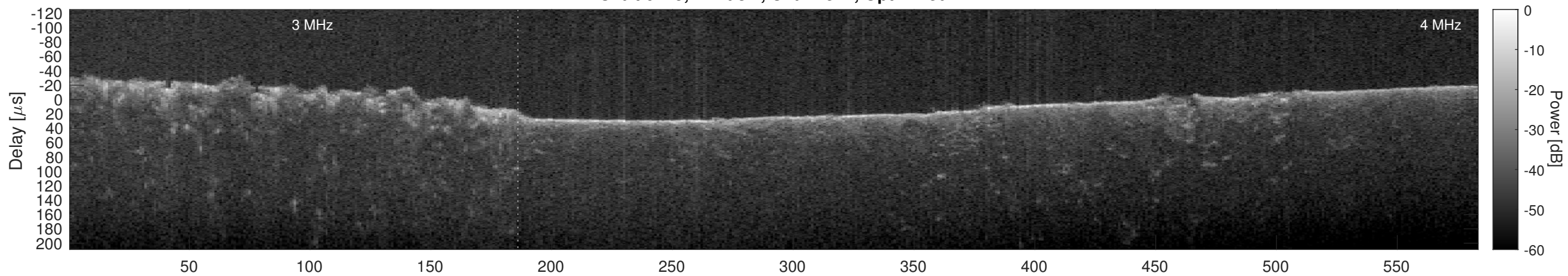
Orbit 6225, Cluttergram
