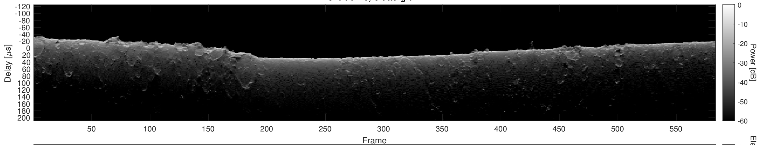
Orbit 6225, Cluttergram
