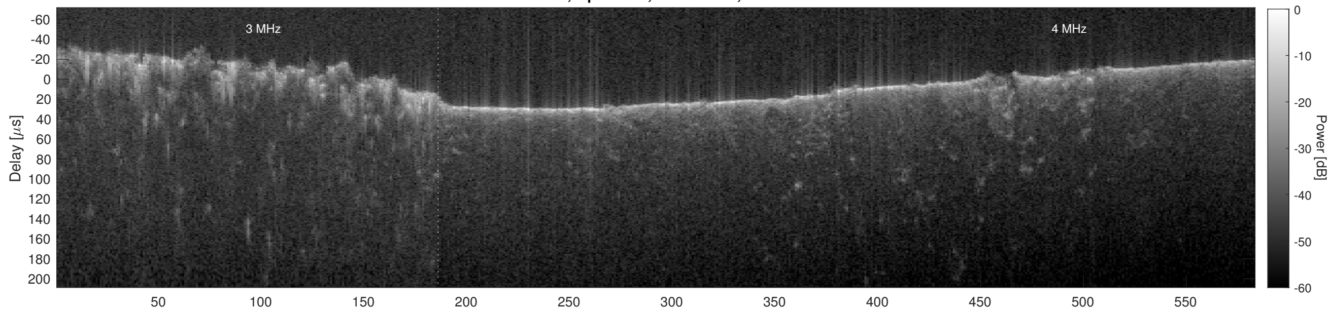
Orbit 6225, Cluttergram
