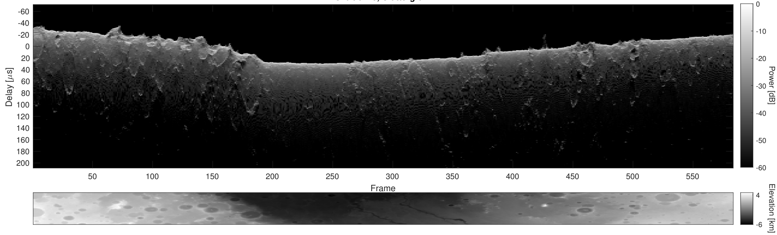
Orbit 6225, Cluttergram
