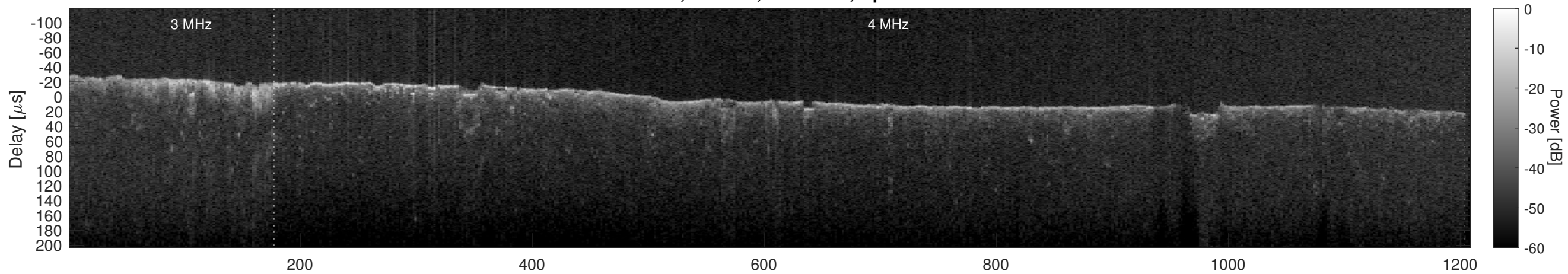
Orbit 6226, Cluttergram
