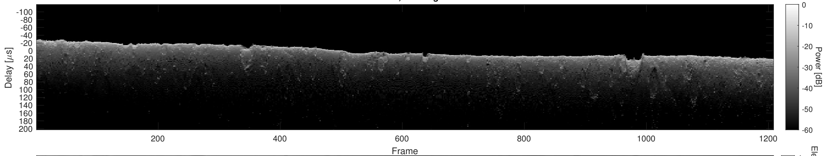
Orbit 6226, Cluttergram
