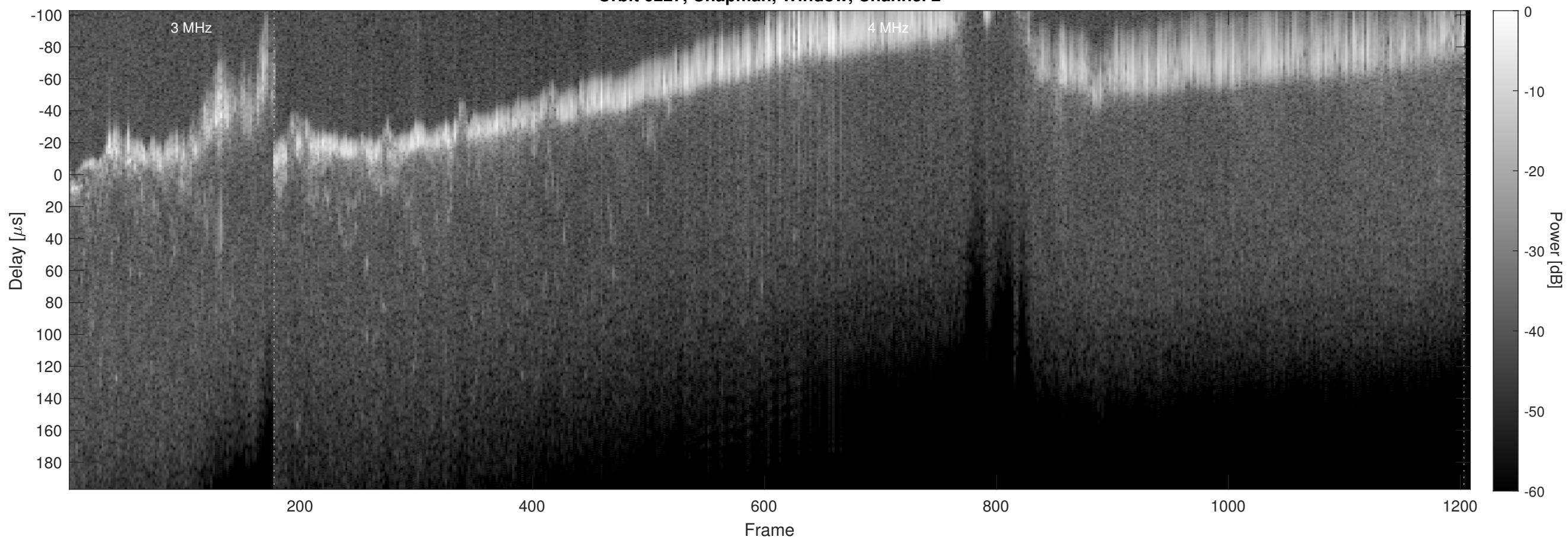
Orbit 6227, Chapman, Window, Channel 2
