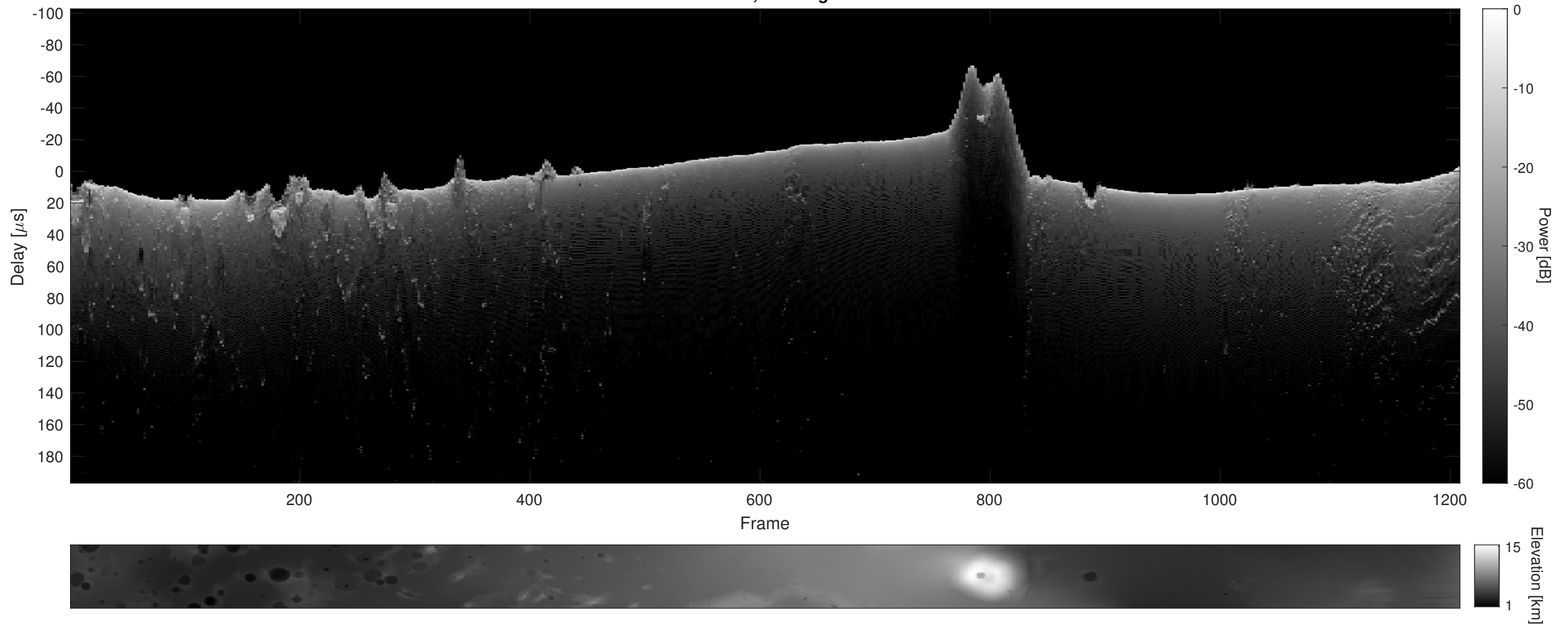
Orbit 6227, Cluttergram
