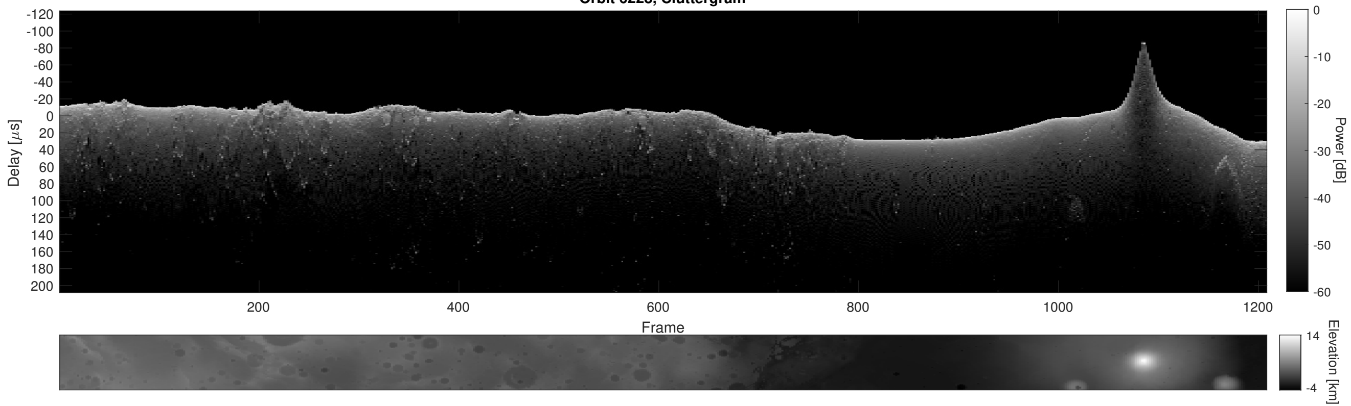
Orbit 6228, Cluttergram
