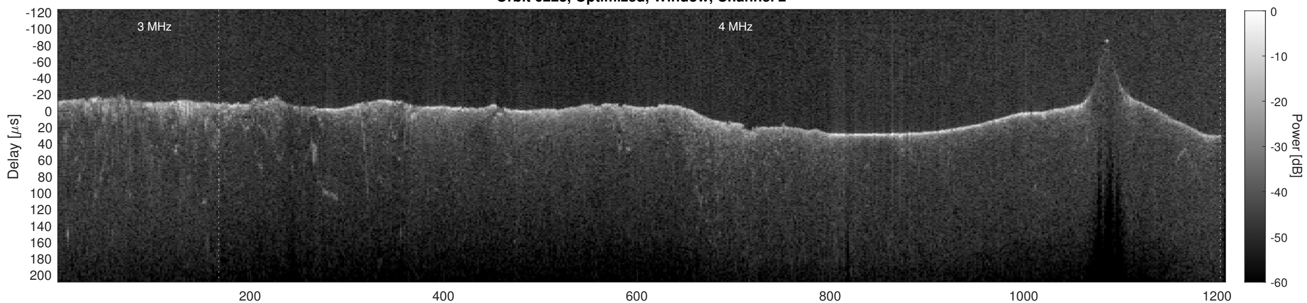
Orbit 6228, Cluttergram
