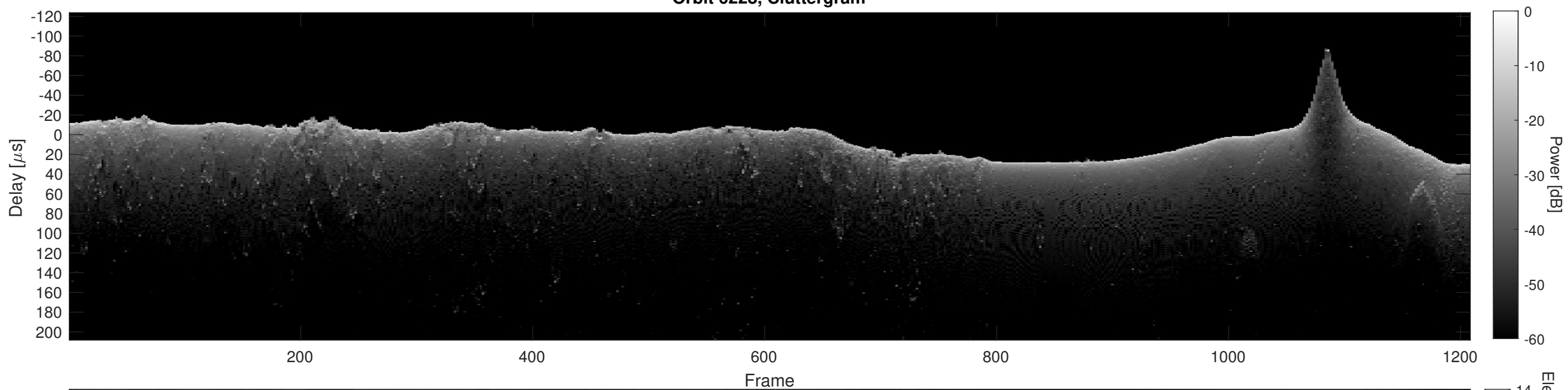
Orbit 6228, Cluttergram
