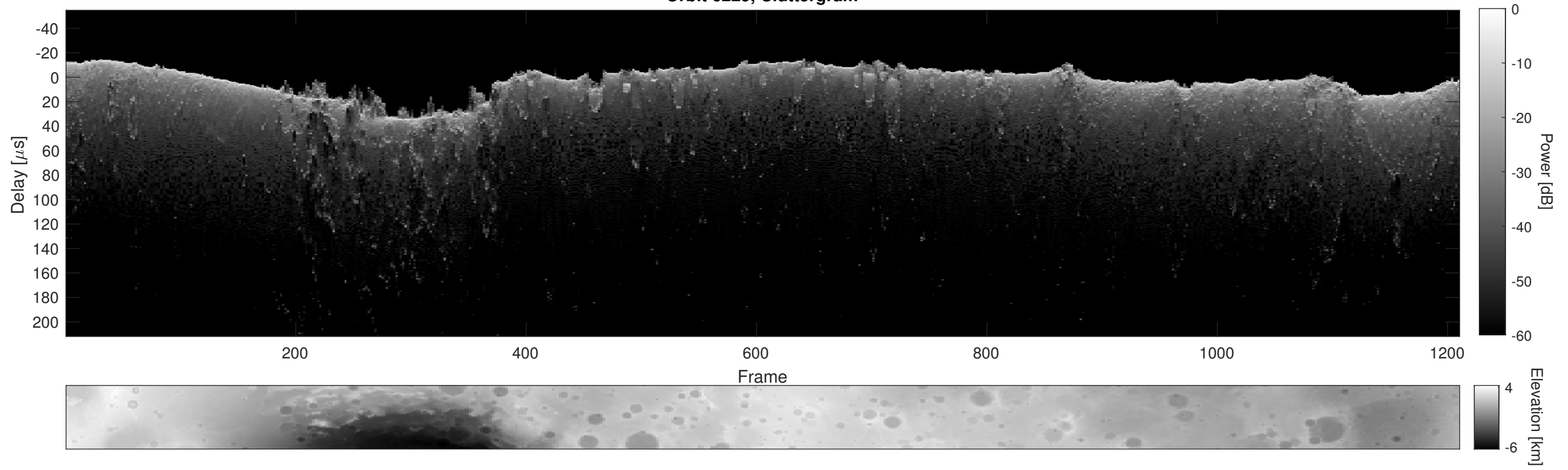
Orbit 6229, Cluttergram
