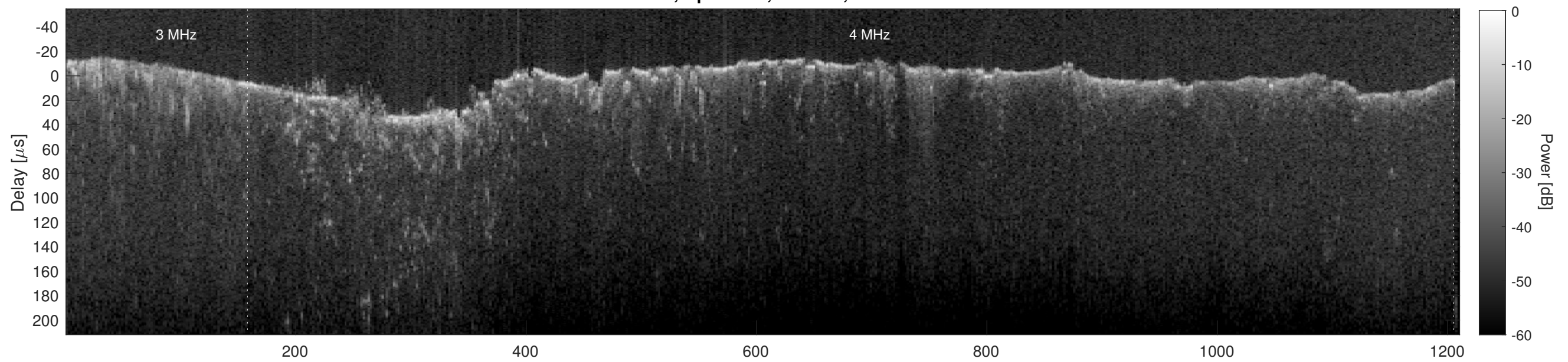
Orbit 6229, Cluttergram
