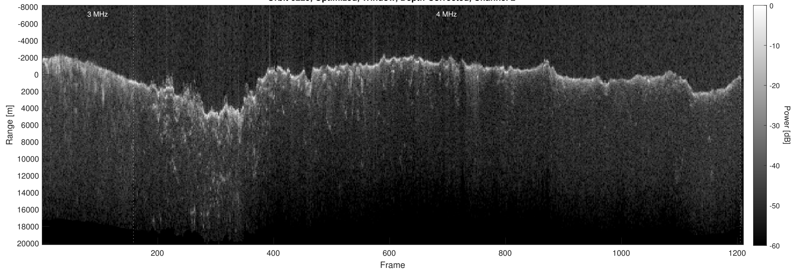
Orbit 6229, Optimized, Window, Depth-Corrected, Channel 2
