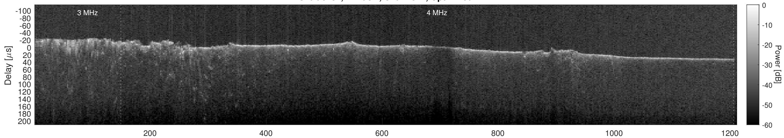
Orbit 6232, Cluttergram
