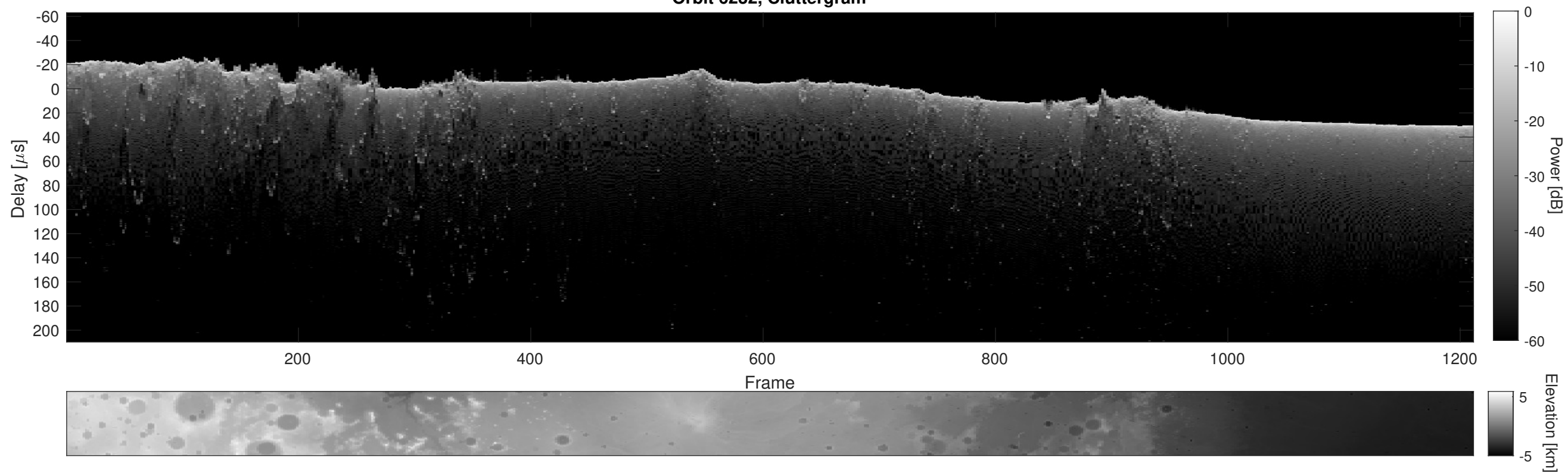
Orbit 6232, Cluttergram
