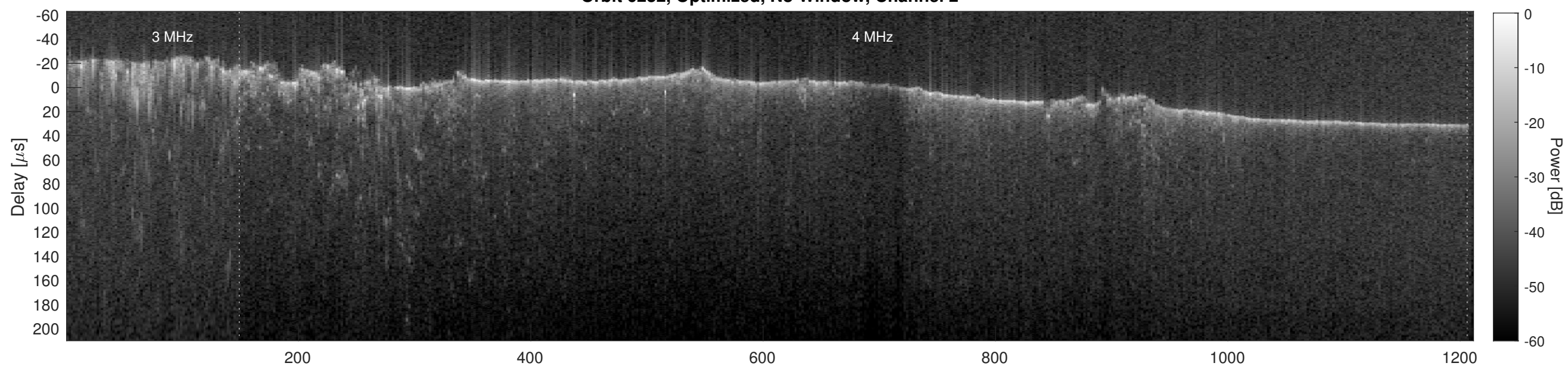
Orbit 6232, Cluttergram
