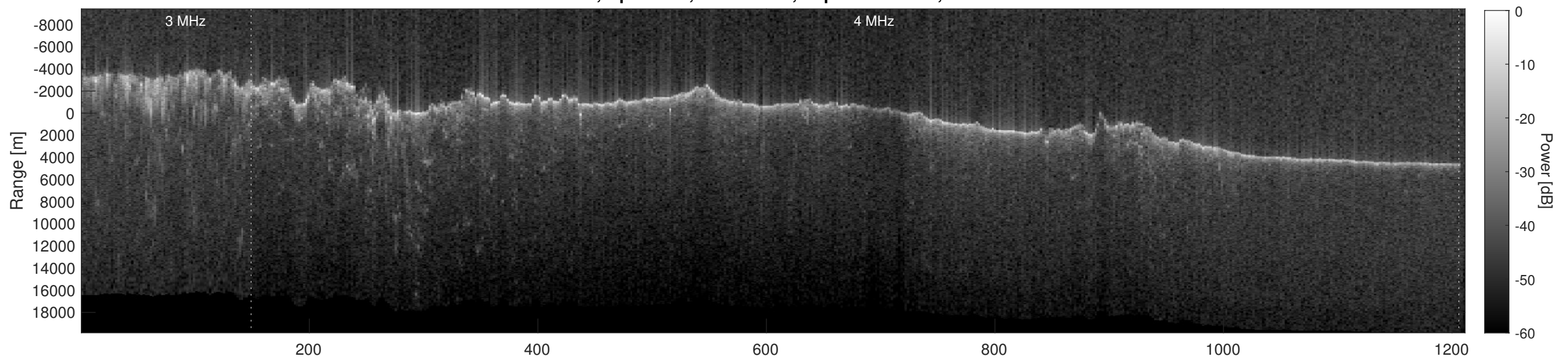
Orbit 6232, Depth-Corrected Cluttergram
