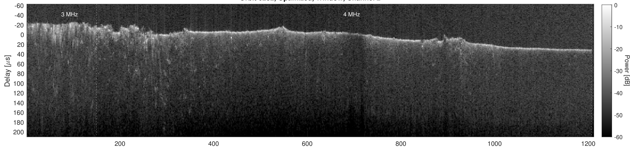
Orbit 6232, Cluttergram
