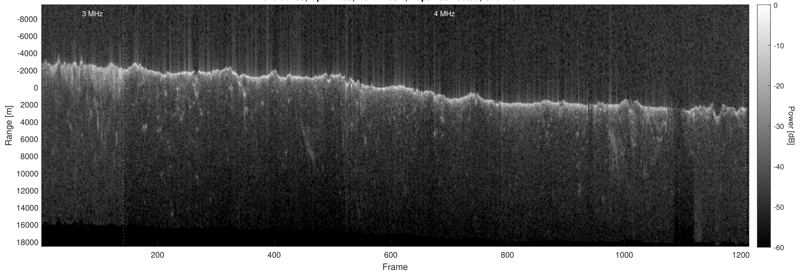
Orbit 6233, Optimized, No Window, Depth-Corrected, Channel 2
