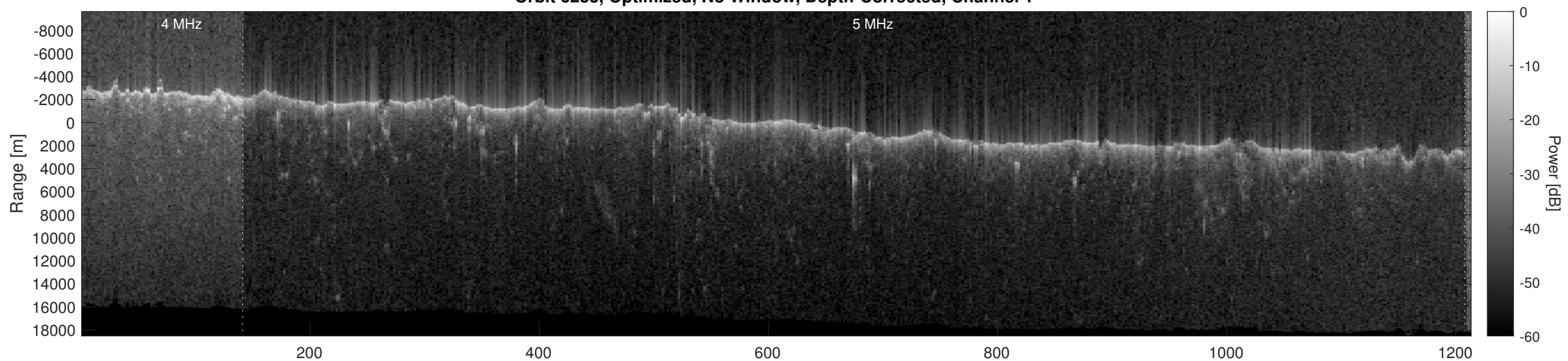
Orbit 6233, Optimized, No Window, Depth-Corrected, Channel 2
