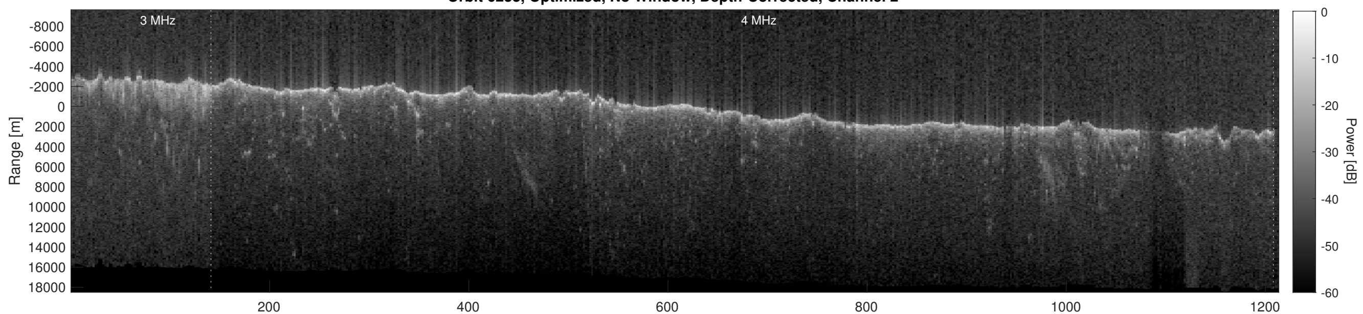
Orbit 6233, Depth-Corrected Cluttergram
