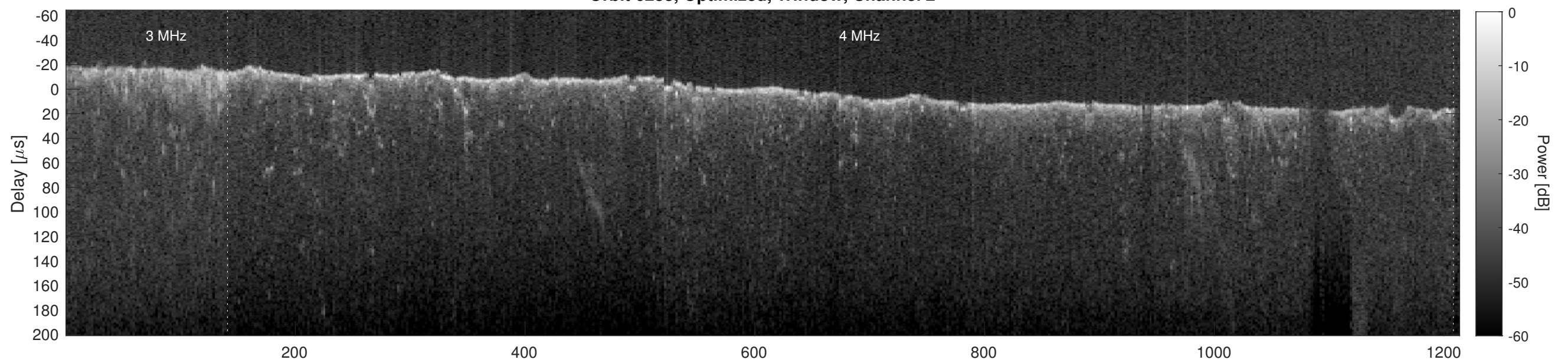
Orbit 6233, Cluttergram
