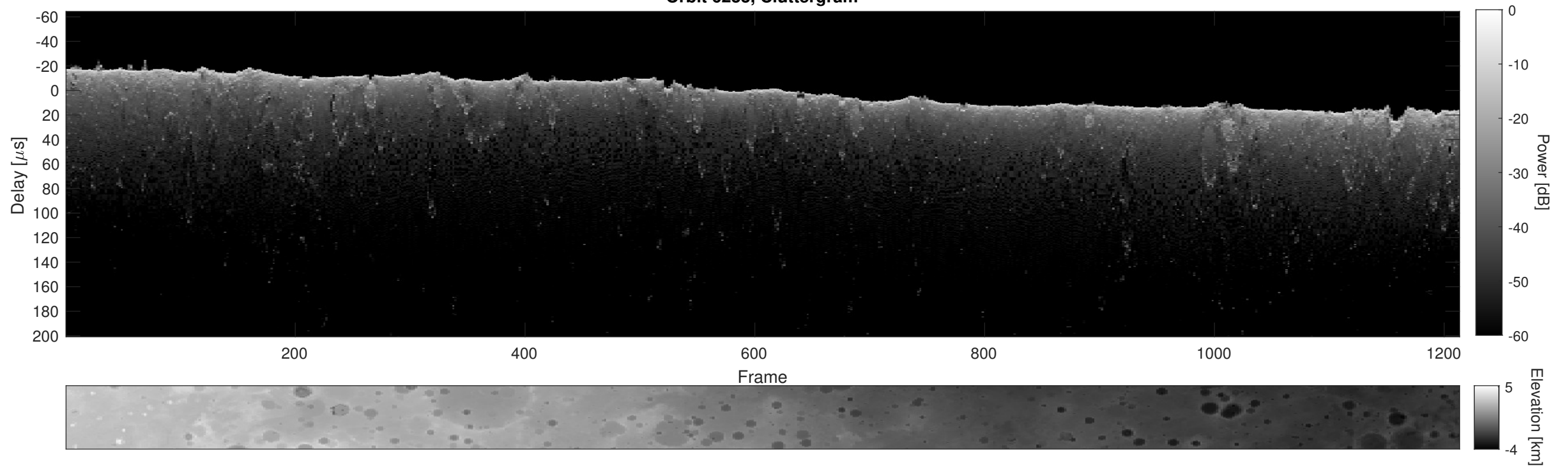
Orbit 6233, Cluttergram
