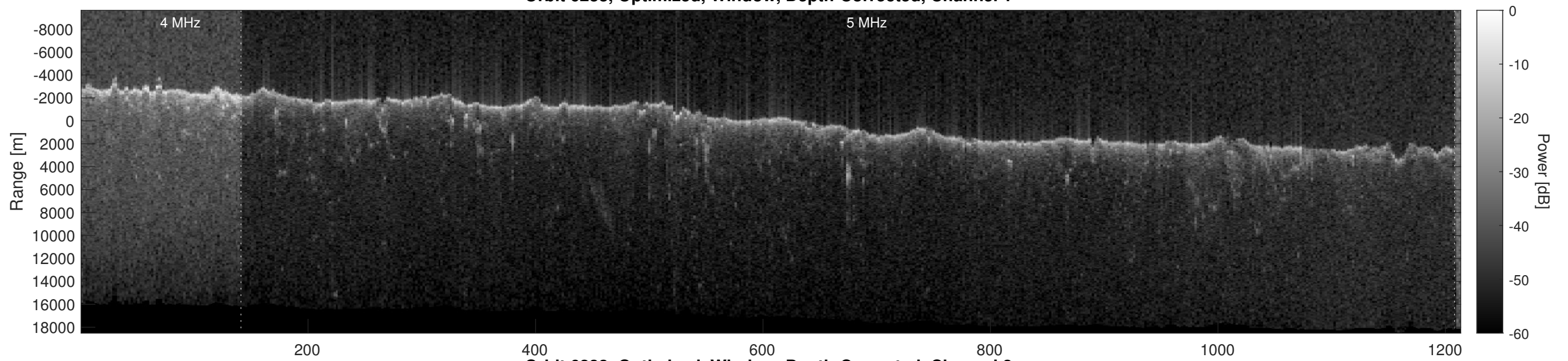
Orbit 6233, Optimized, Window, Depth-Corrected, Channel 2
