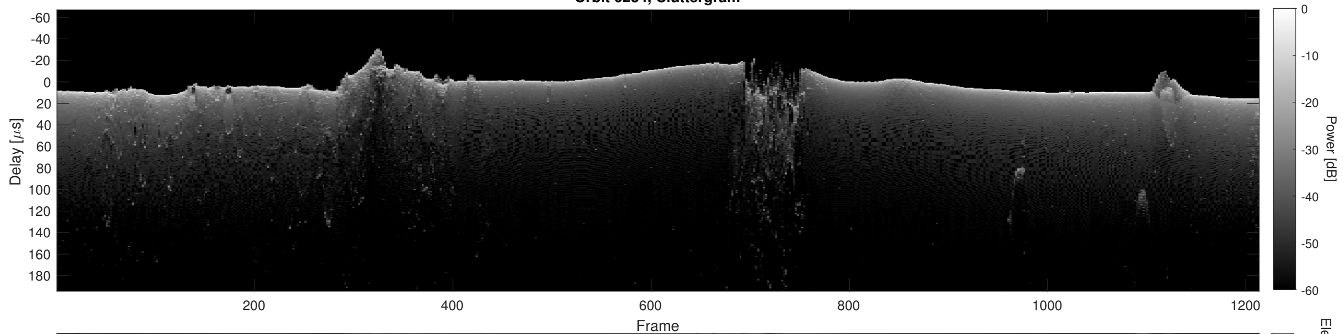
Orbit 6234, Cluttergram
