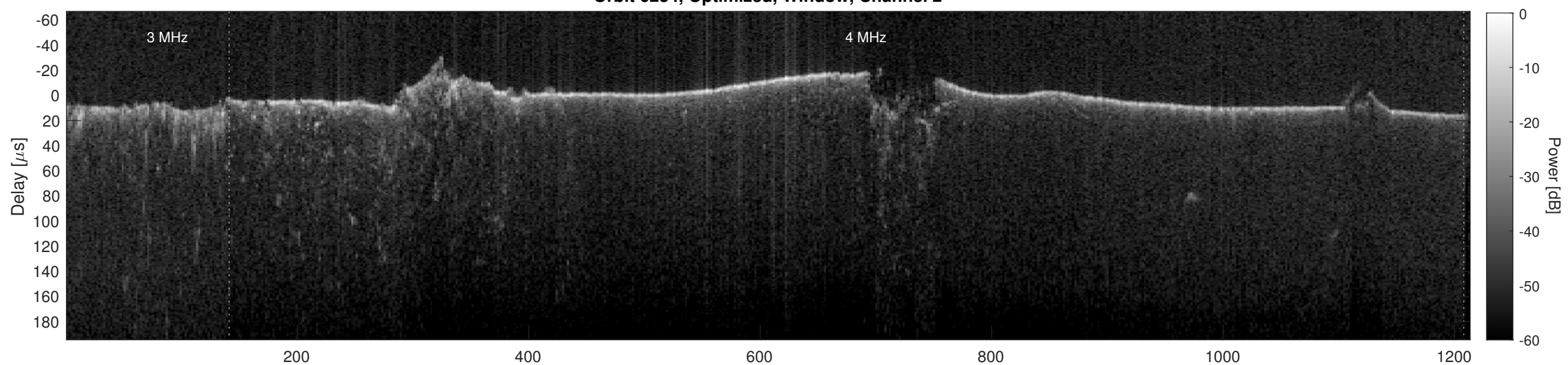
Orbit 6234, Cluttergram
