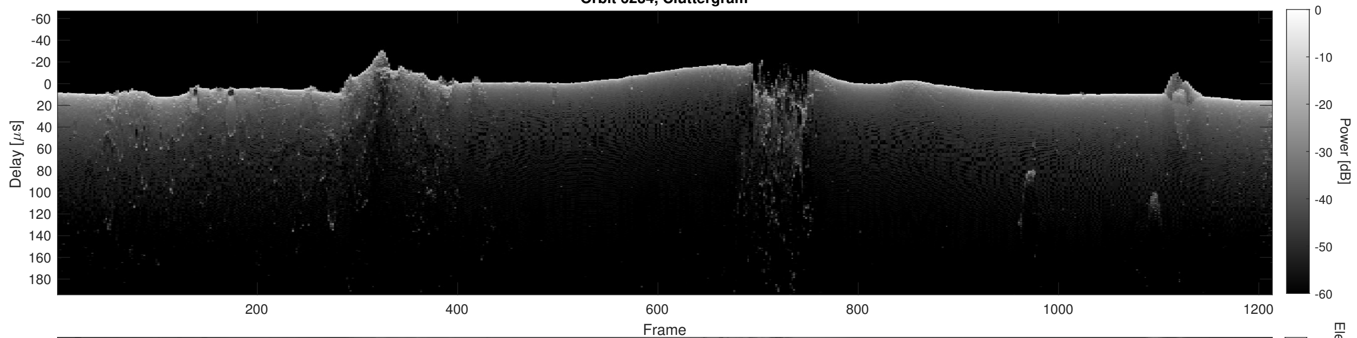
Orbit 6234, Cluttergram
