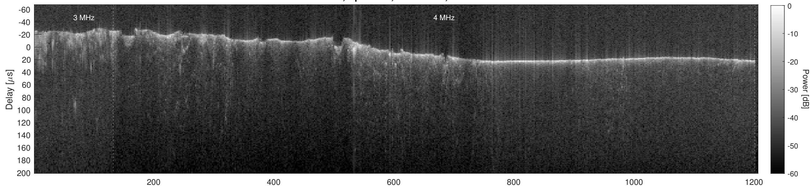
Orbit 6235, Cluttergram
