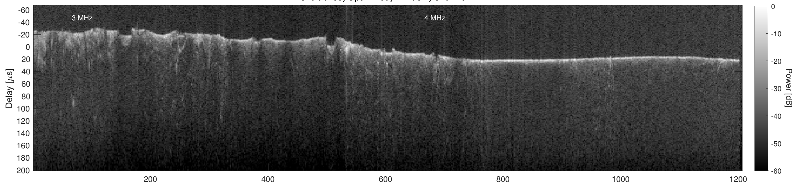
Orbit 6235, Cluttergram
