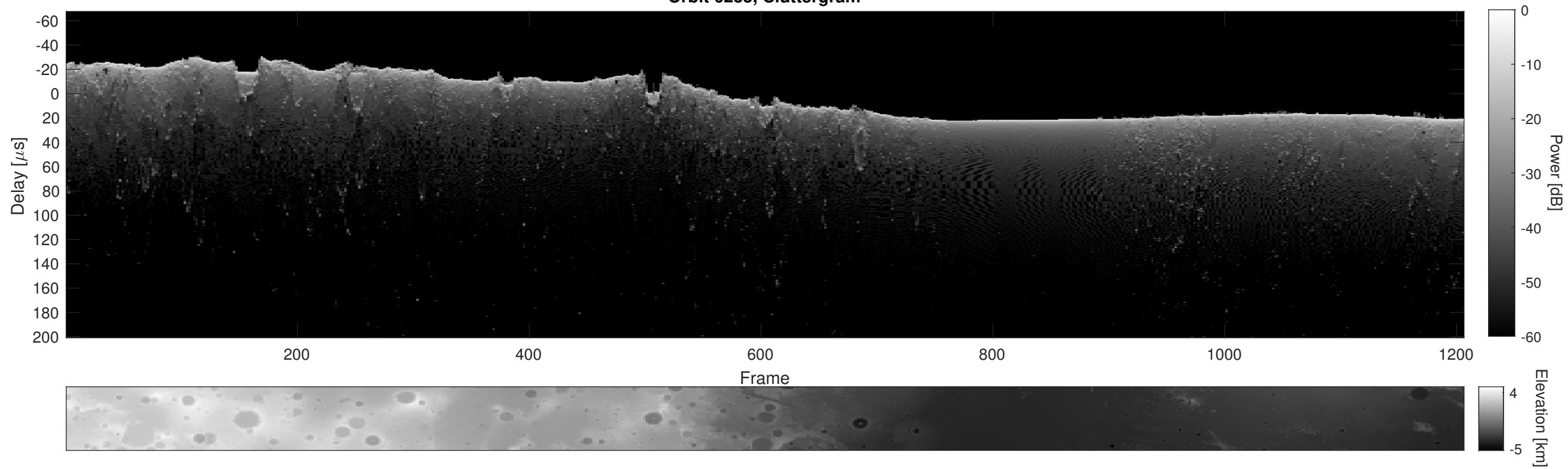
Orbit 6235, Cluttergram
