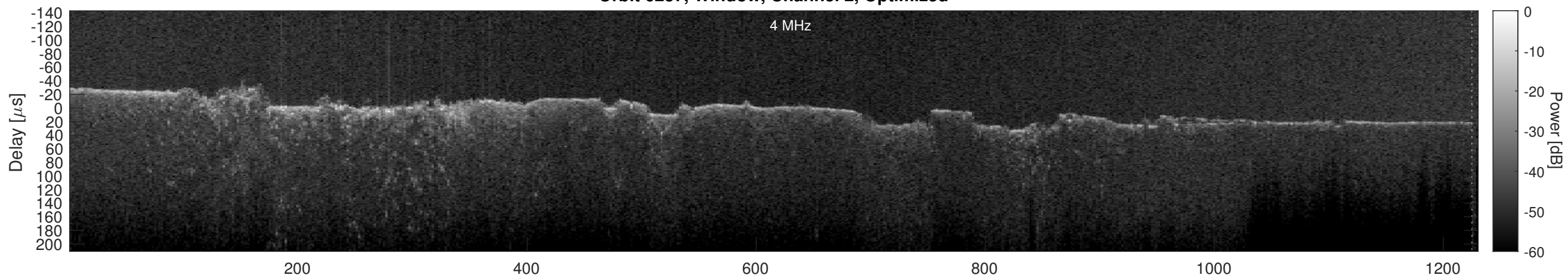
Orbit 6237, Cluttergram
