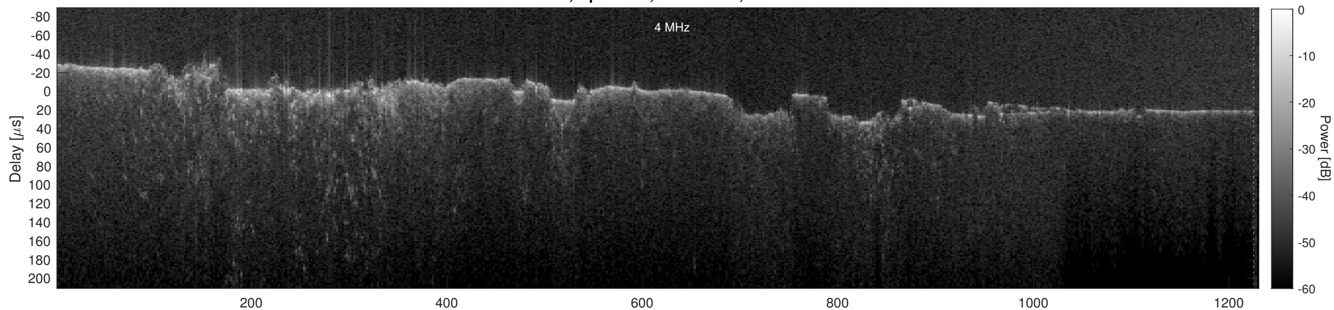
Orbit 6237, Cluttergram
