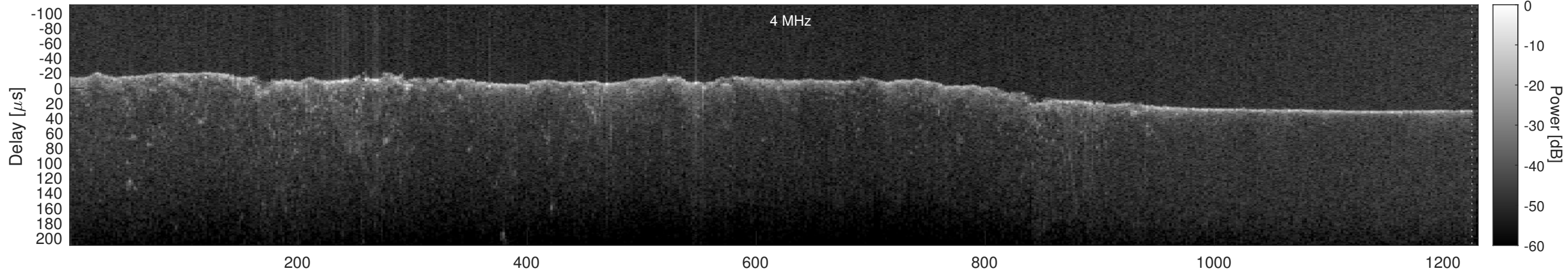
Orbit 6239, Cluttergram
