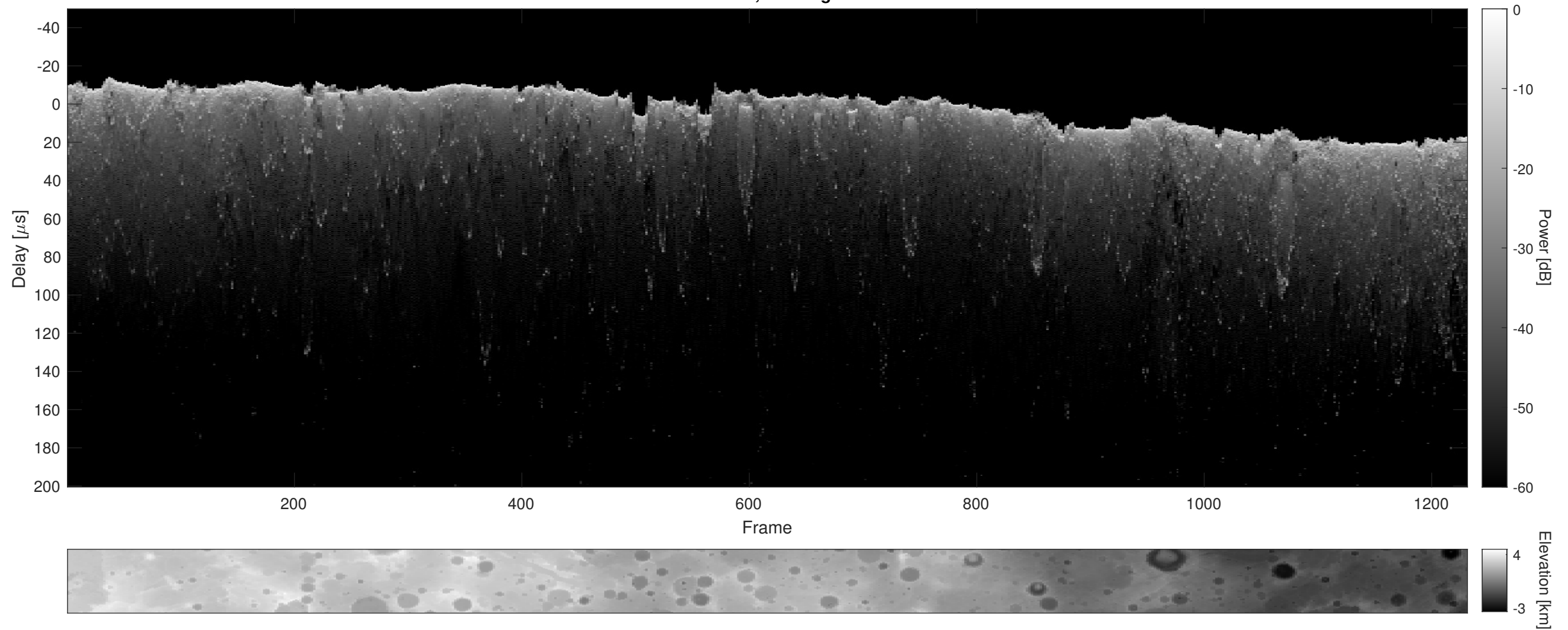
Orbit 6240, Cluttergram
