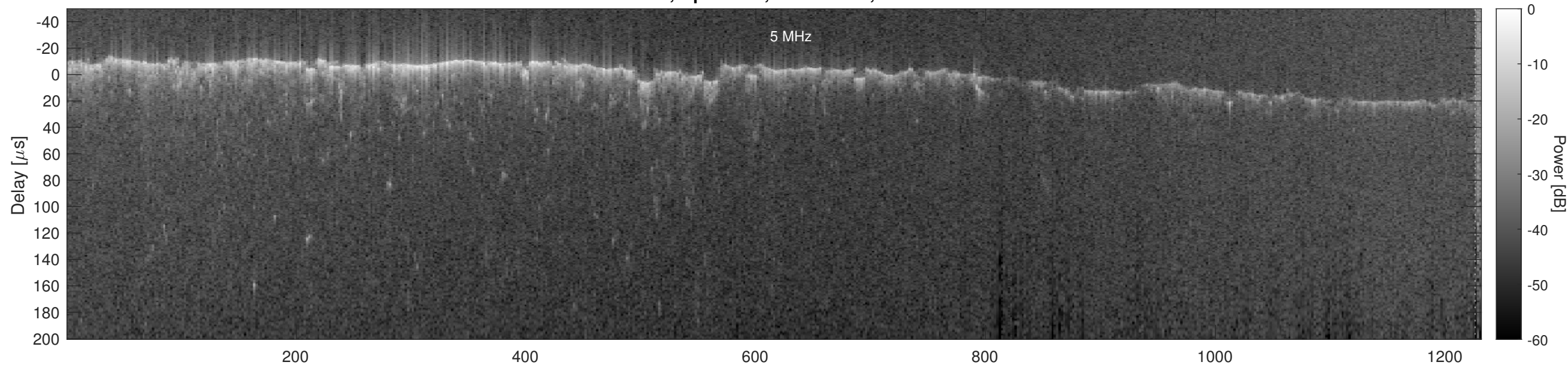
Orbit 6240, Optimized, No Window, Channel 2
