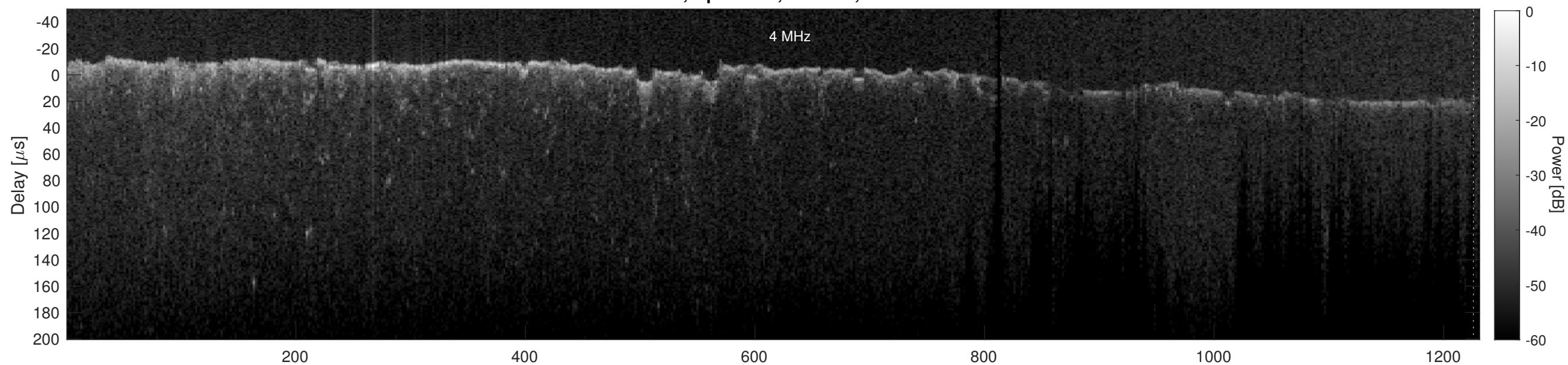
Orbit 6240, Cluttergram
