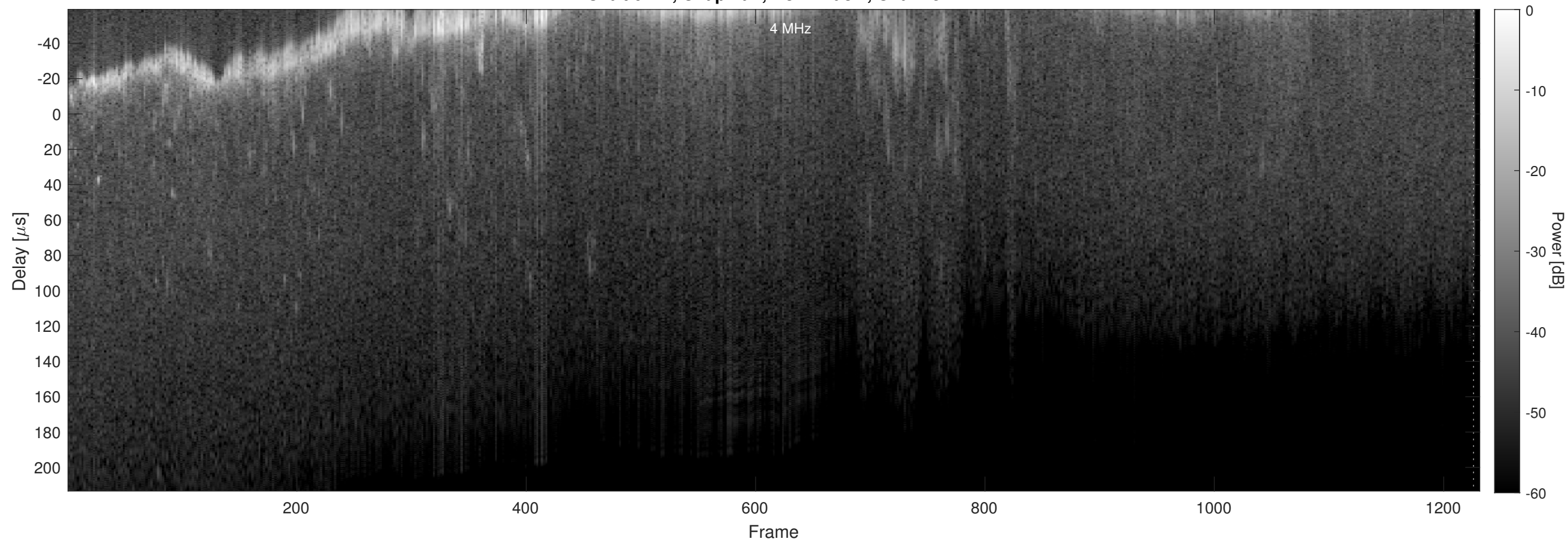
Orbit 6241, Chapman, No Window, Channel 2
