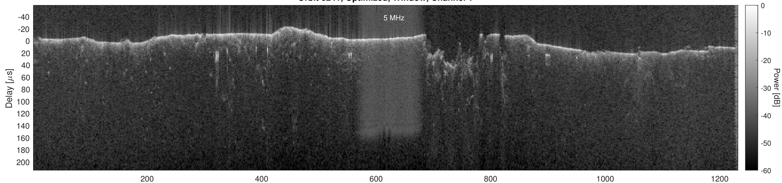
Orbit 6241, Optimized, Window, Channel 2
