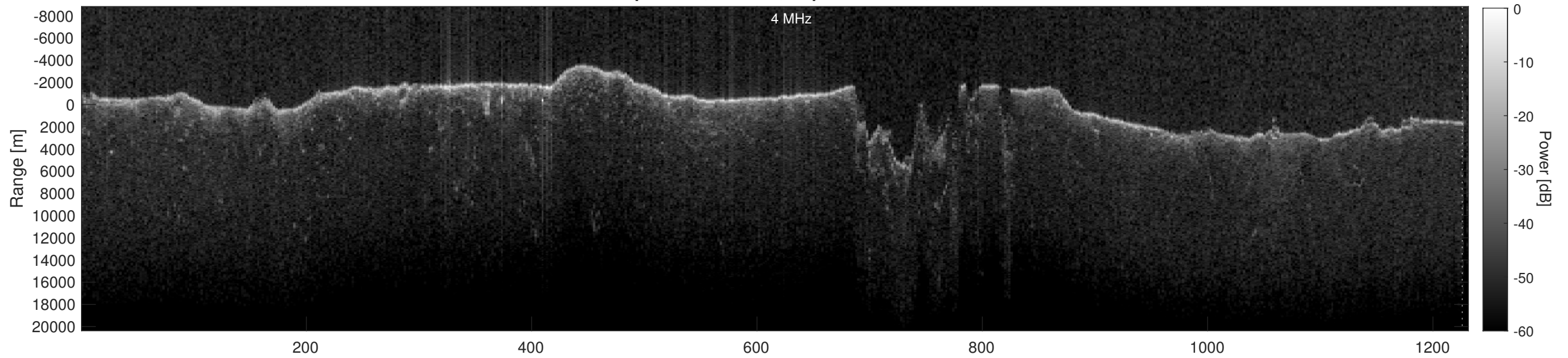
Orbit 6241, Depth-Corrected Cluttergram
