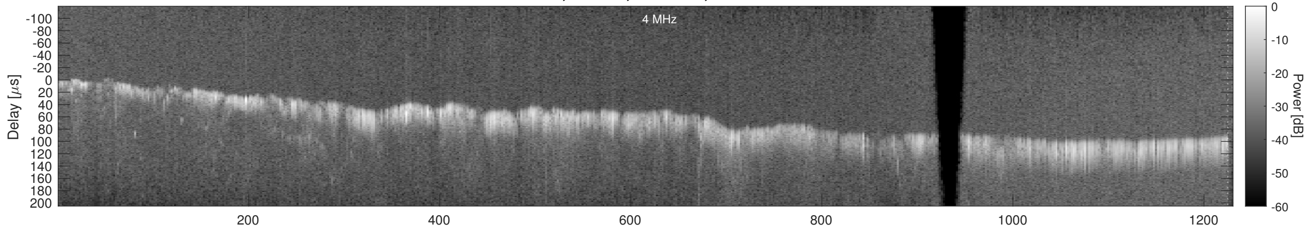
Orbit 6242, Window, Channel 2, Chapman
