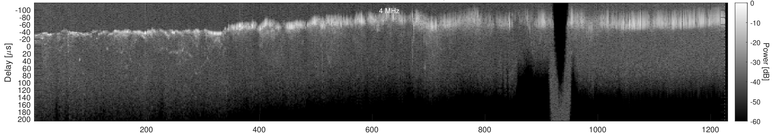
Orbit 6242, Window, Channel 2, Optimized
