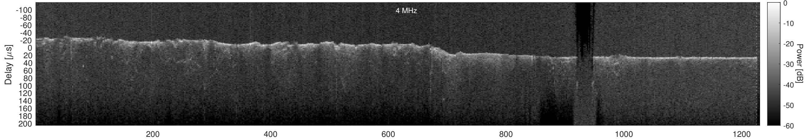
Orbit 6242, Cluttergram
