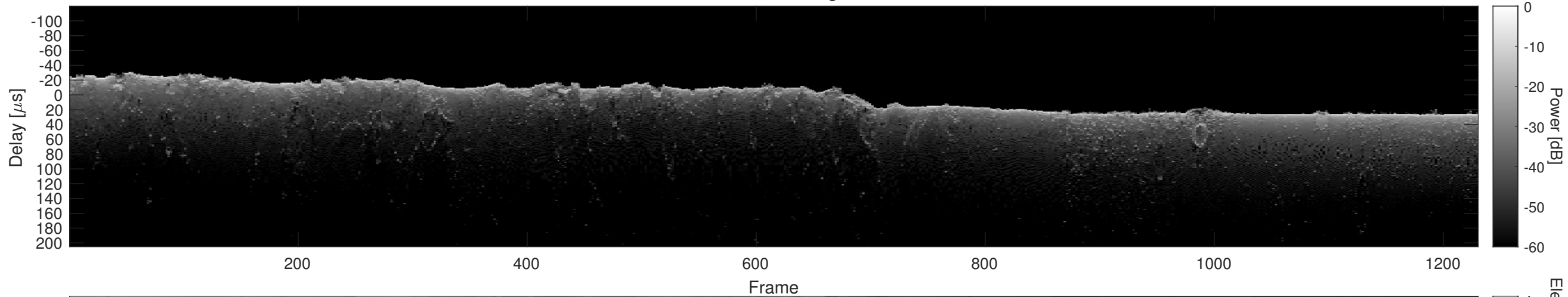
Orbit 6242, Cluttergram
