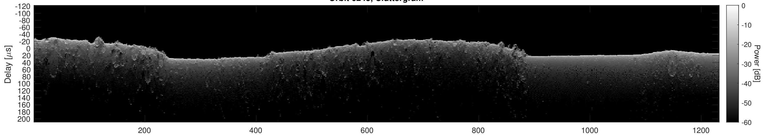
Orbit 6243, Cluttergram
