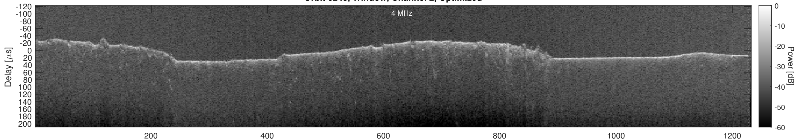
Orbit 6243, Cluttergram
