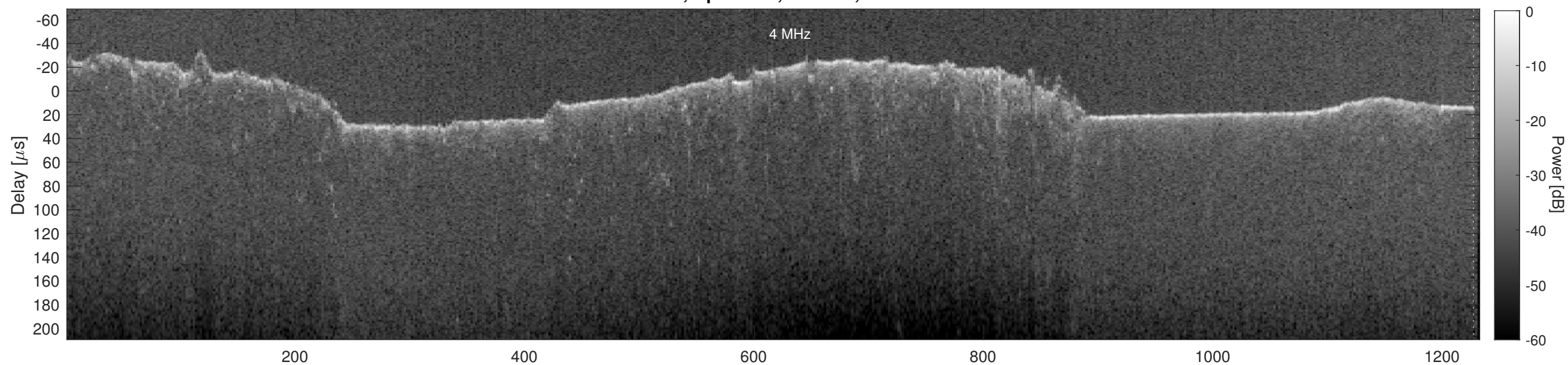
Orbit 6243, Cluttergram
