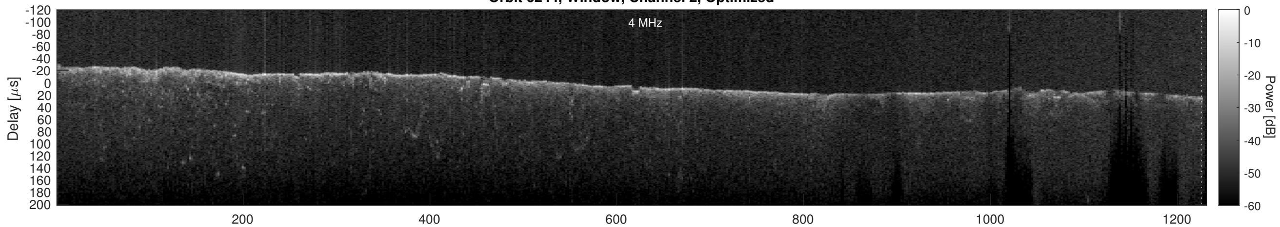
Orbit 6244, Cluttergram
