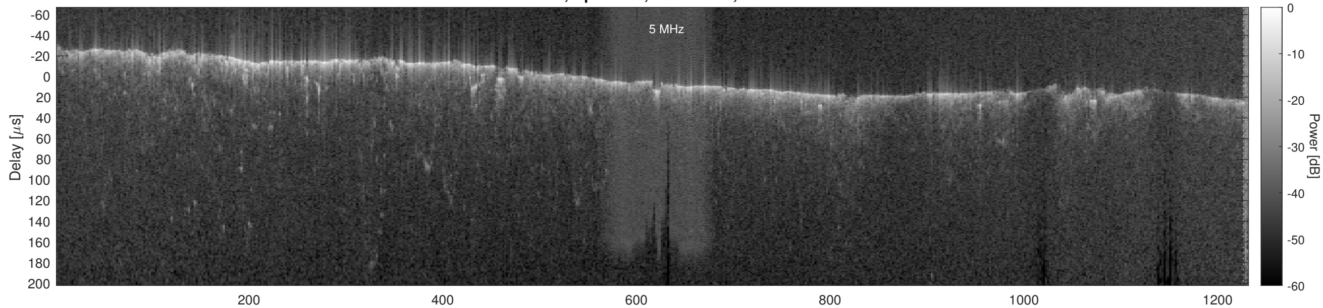
Orbit 6244, Optimized, No Window, Channel 2
