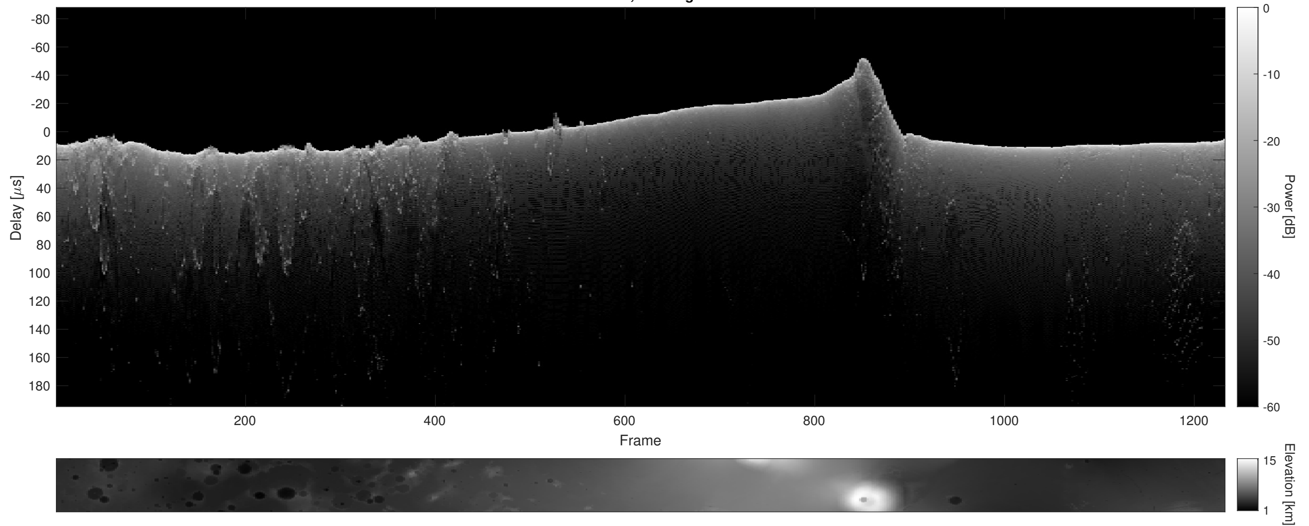
Orbit 6245, Cluttergram
