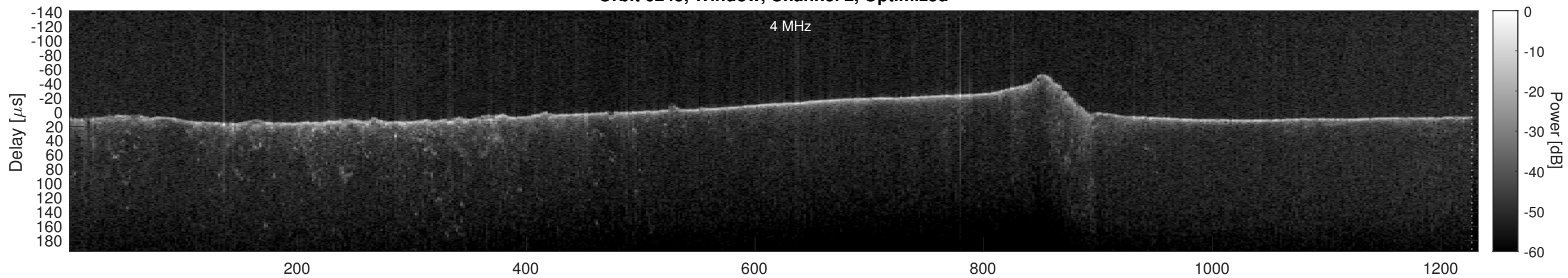
Orbit 6245, Cluttergram
