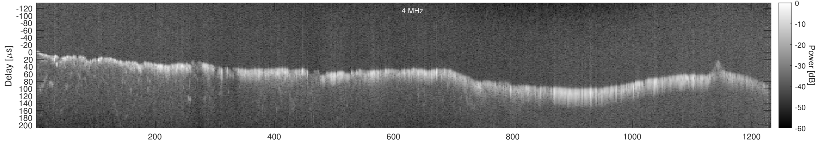
Orbit 6246, Window, Channel 2, Chapman
