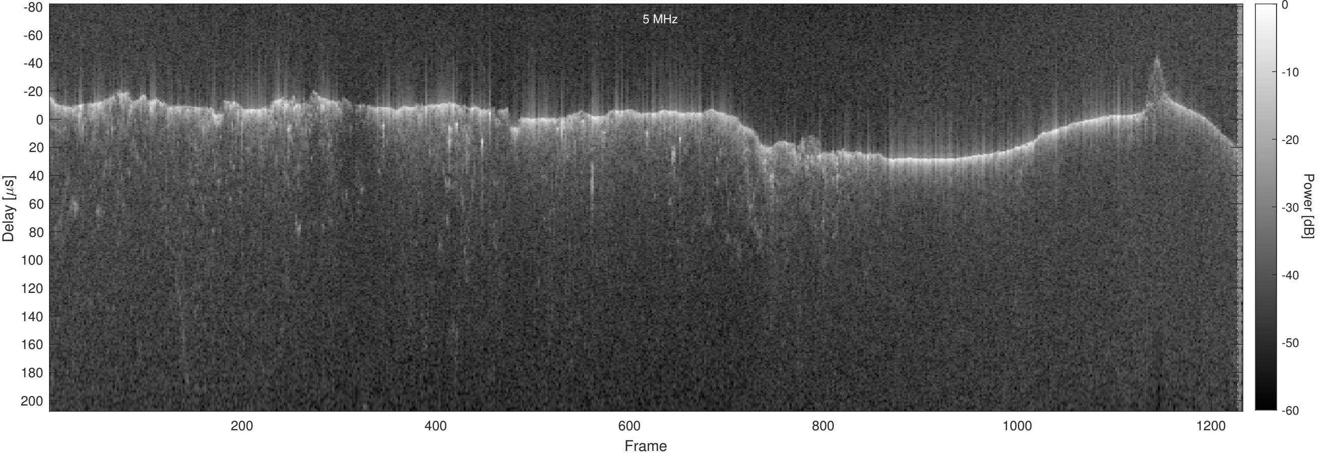
Orbit 6246, Optimized, No Window, Channel 2
