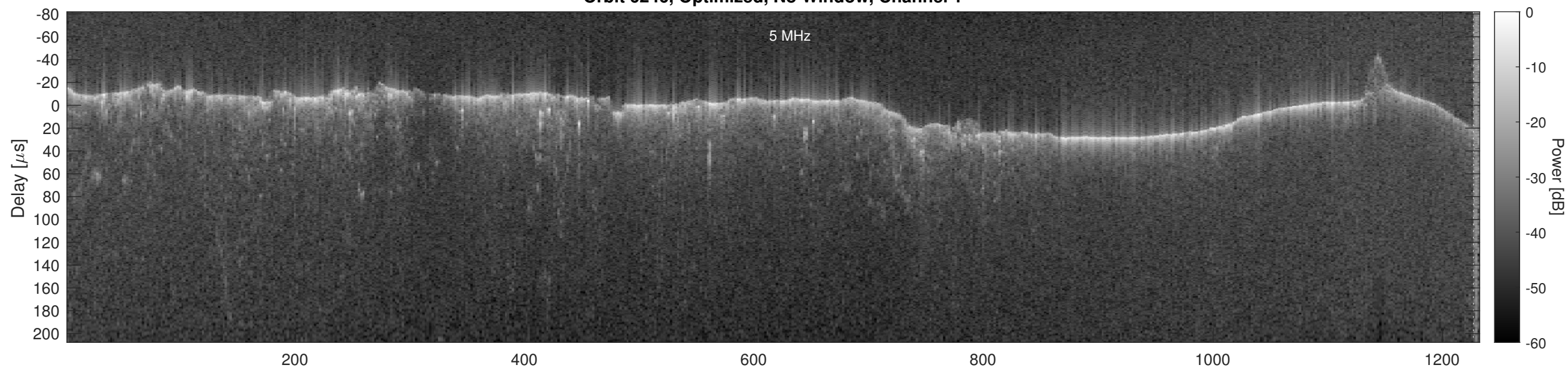
Orbit 6246, Optimized, No Window, Channel 2
