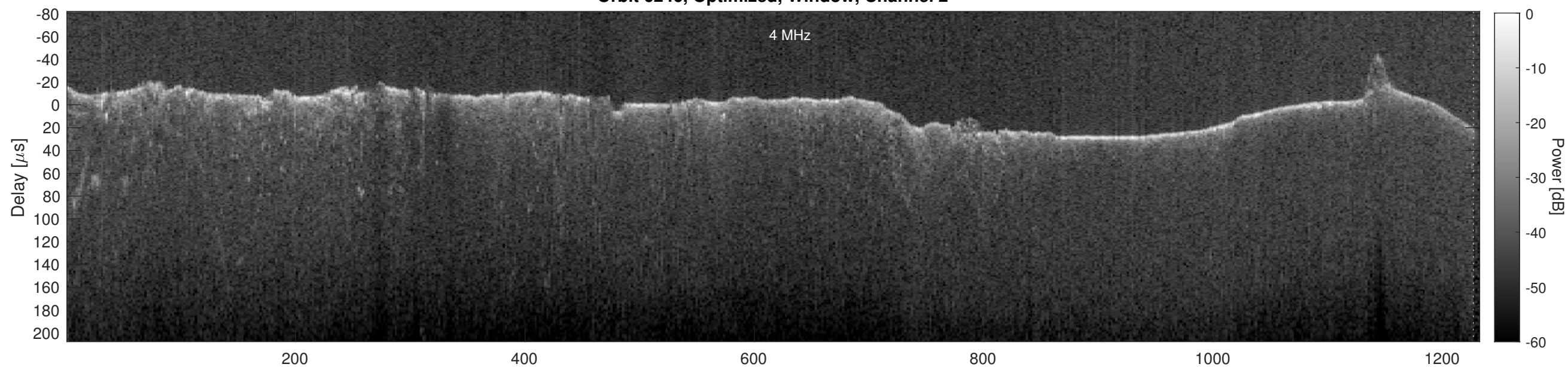
Orbit 6246, Cluttergram
