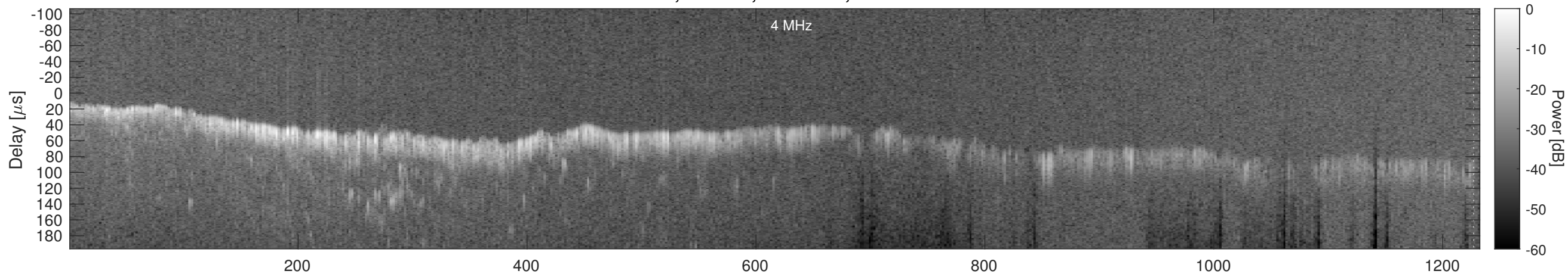
Orbit 6247, Window, Channel 2, Chapman
