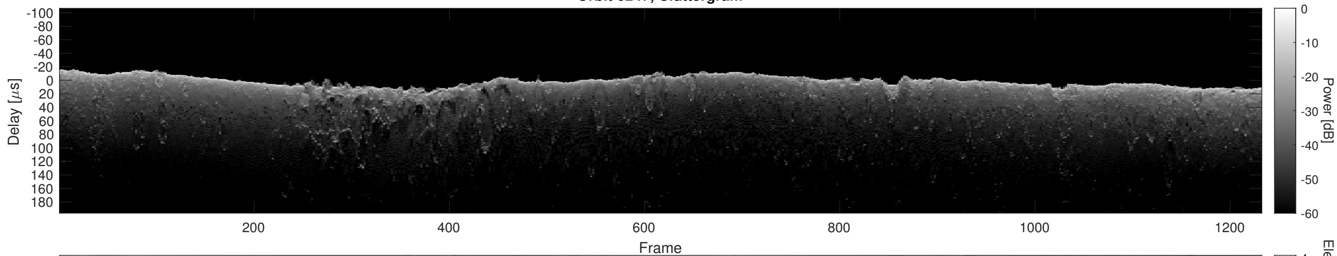
Orbit 6247, Cluttergram
