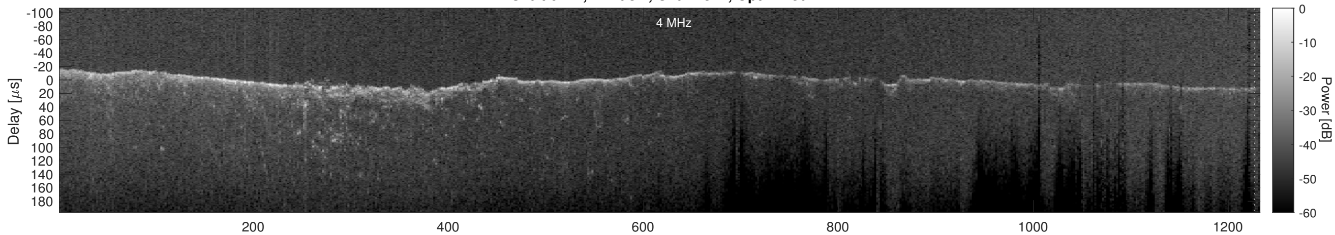
Orbit 6247, Cluttergram
