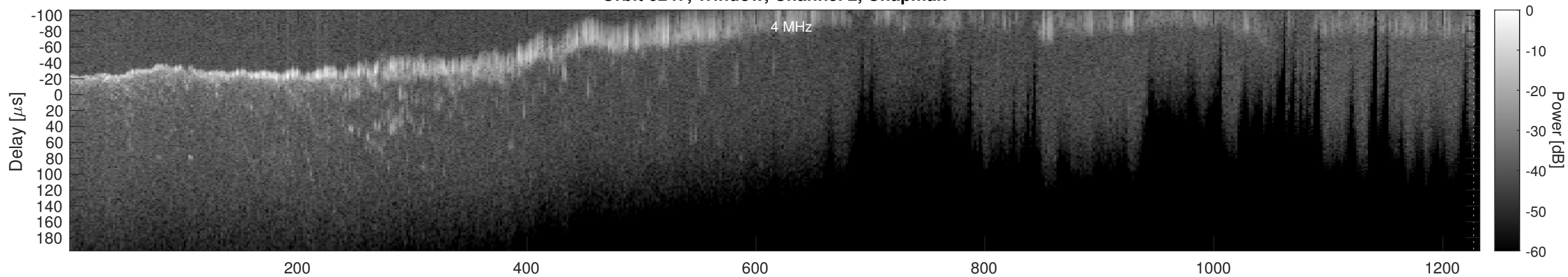
Orbit 6247, Window, Channel 2, Optimized
