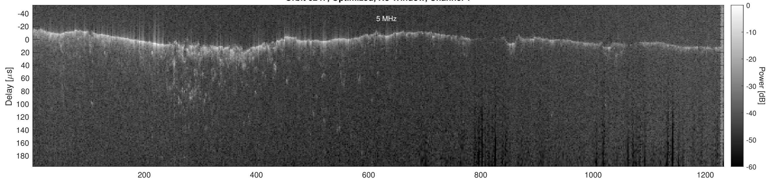
Orbit 6247, Optimized, No Window, Channel 2
