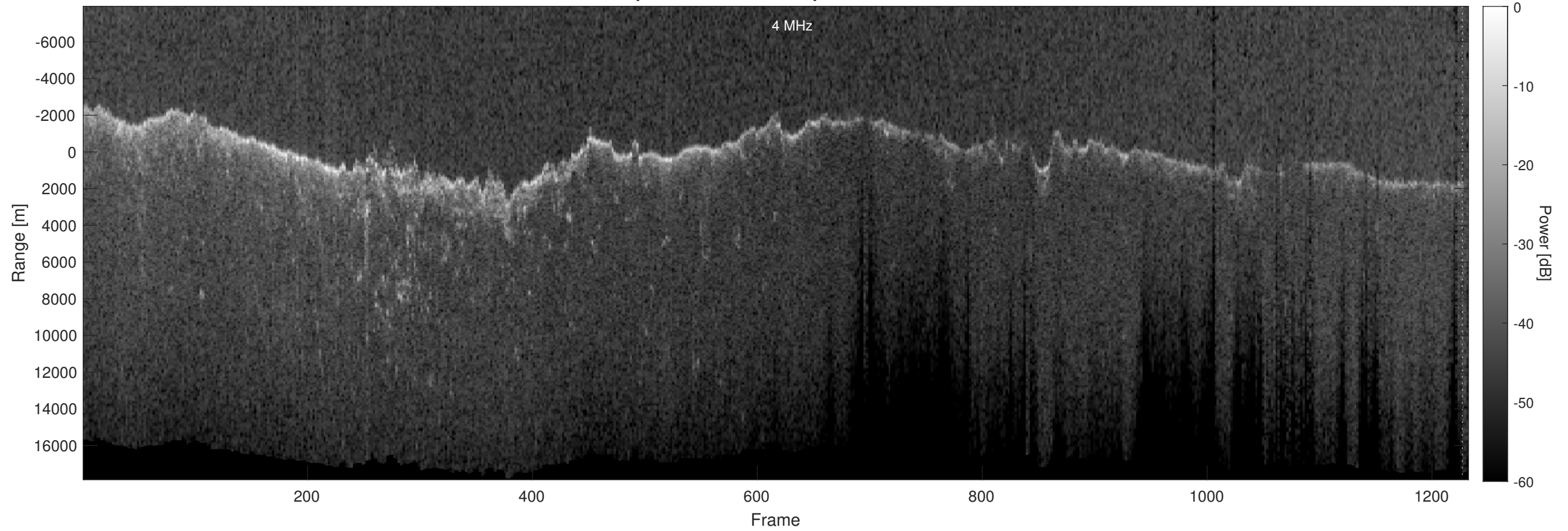
Orbit 6247, Optimized, Window, Depth-Corrected, Channel 2
