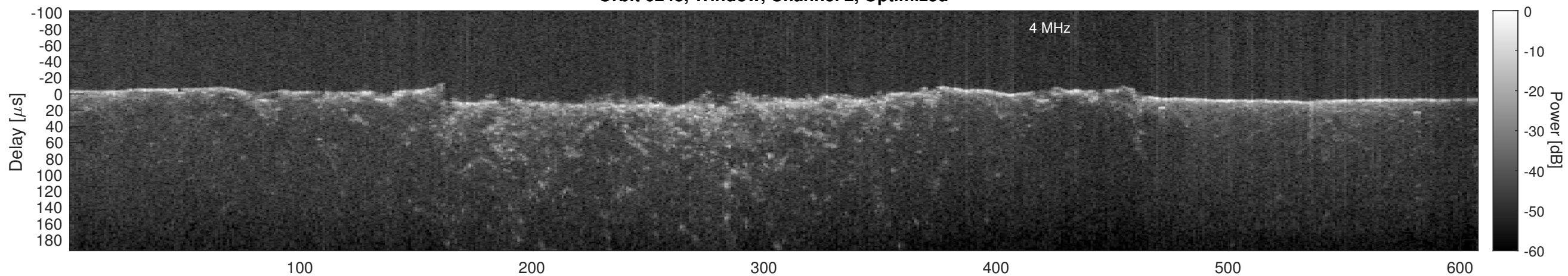
Orbit 6248, Cluttergram
