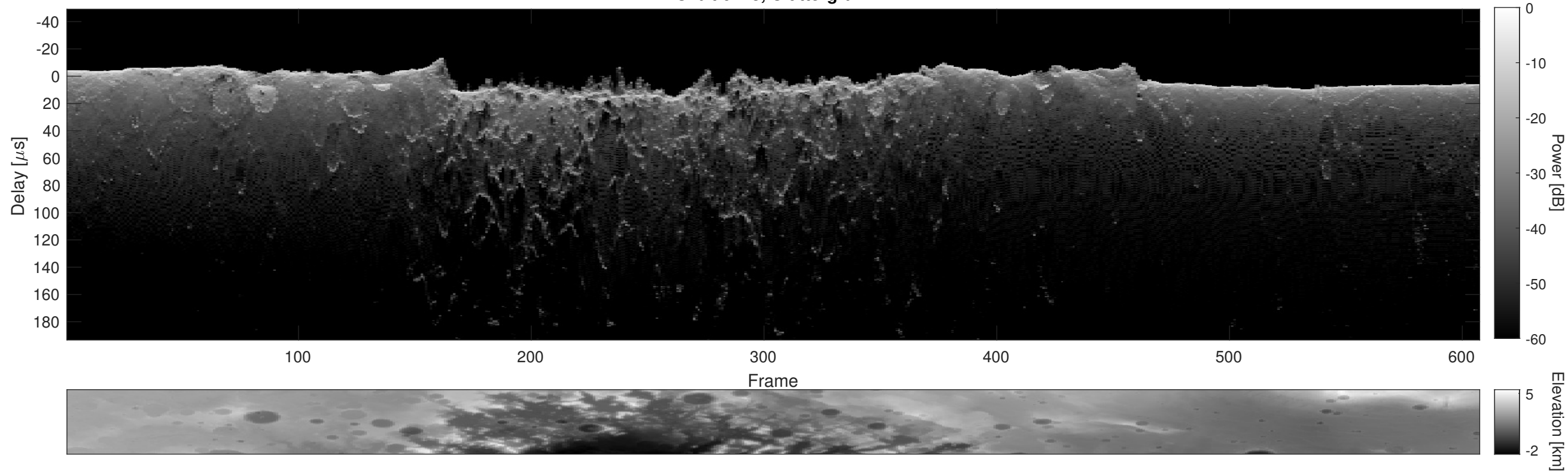
Orbit 6248, Cluttergram
