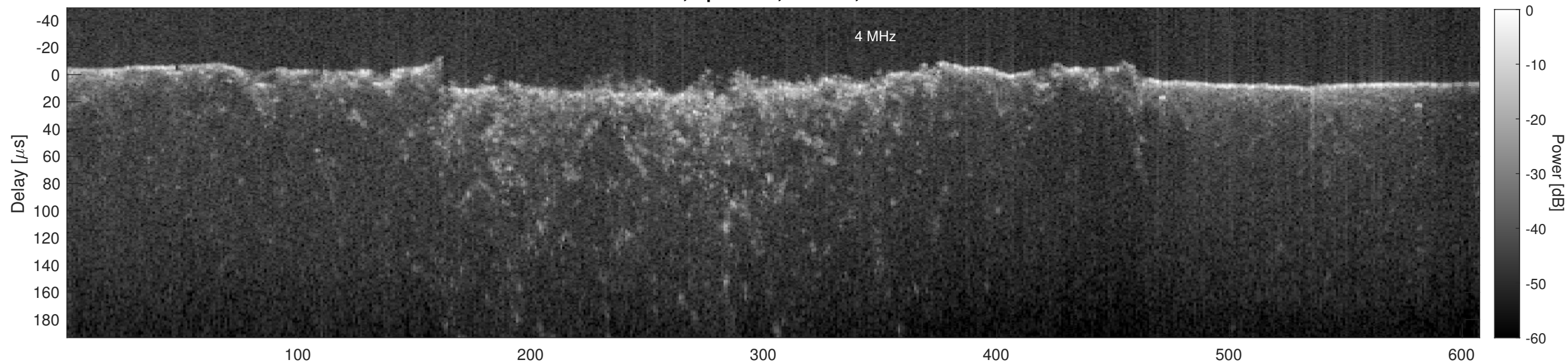
Orbit 6248, Cluttergram
